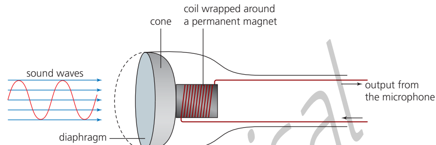
▲ Figure 3.15 Diagram of how a microphone works
