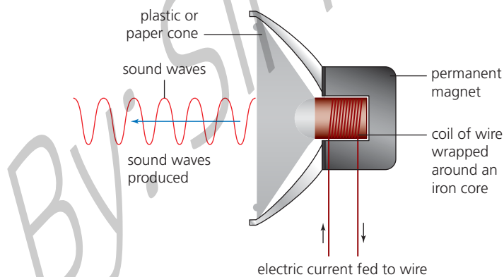
▲ Figure 3.14 Diagram showing how a loudspeaker works
