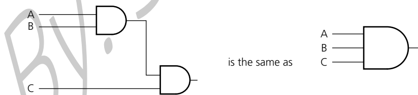
▲ Figure 3.32 Multi-input AND gate
