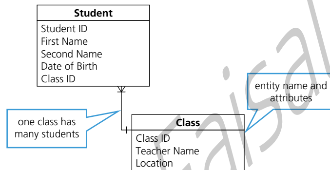
▲ Figure 8.3 E-R diagram for school database
